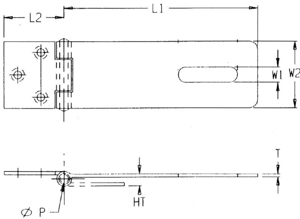
Stainless Steel Hasp
