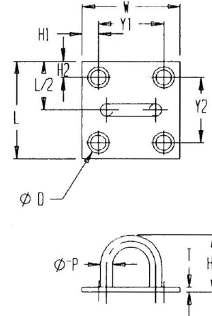
Stainless Steel Staple
